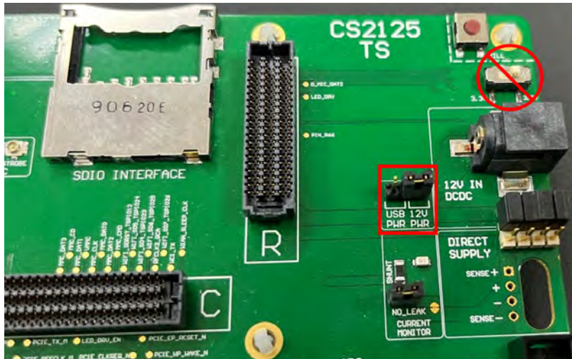
Figure 18: EVB 2.0 Jumper Setting for DC-DC mode
