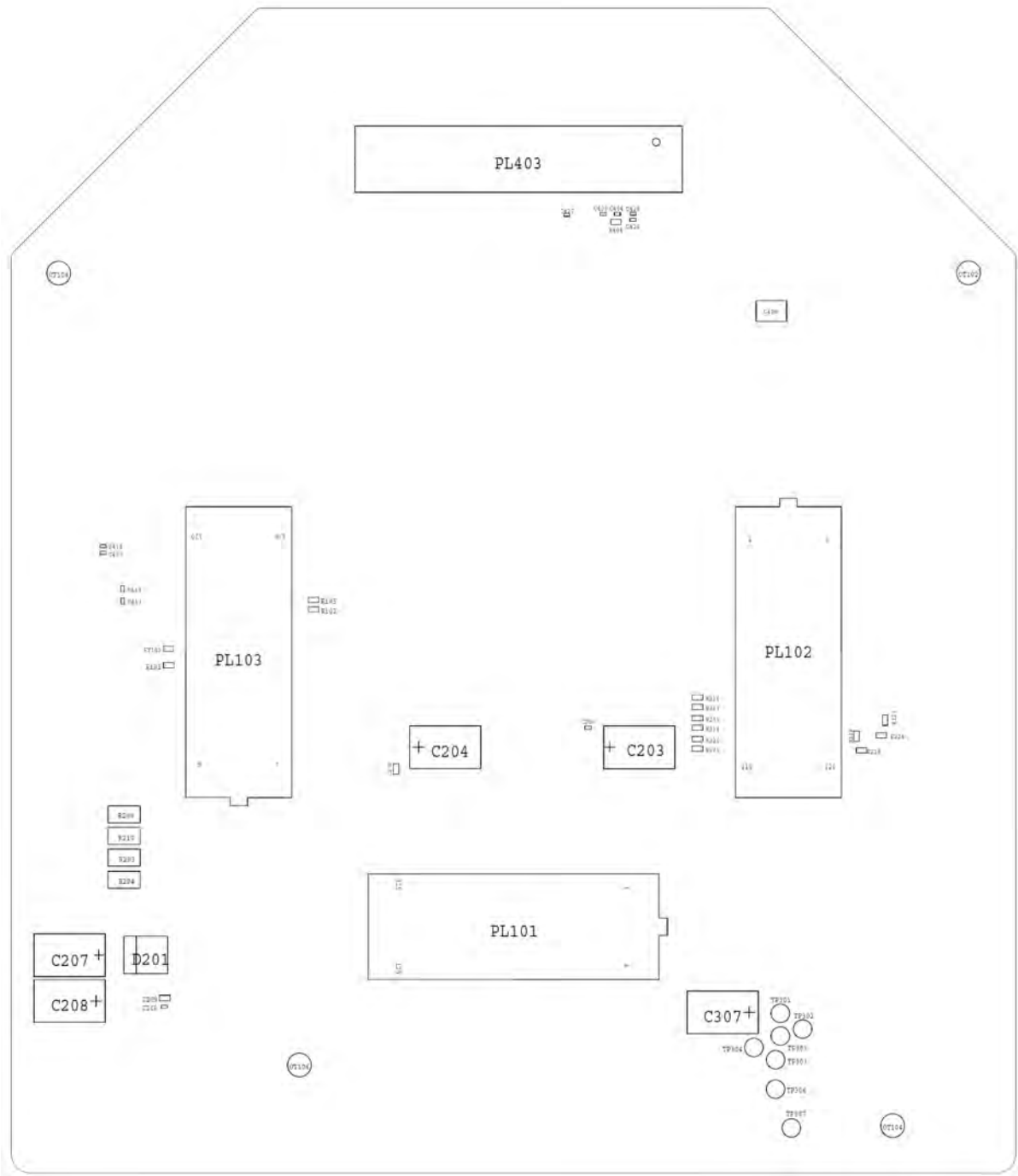
Figure 23: Component Diagram Bottom View
