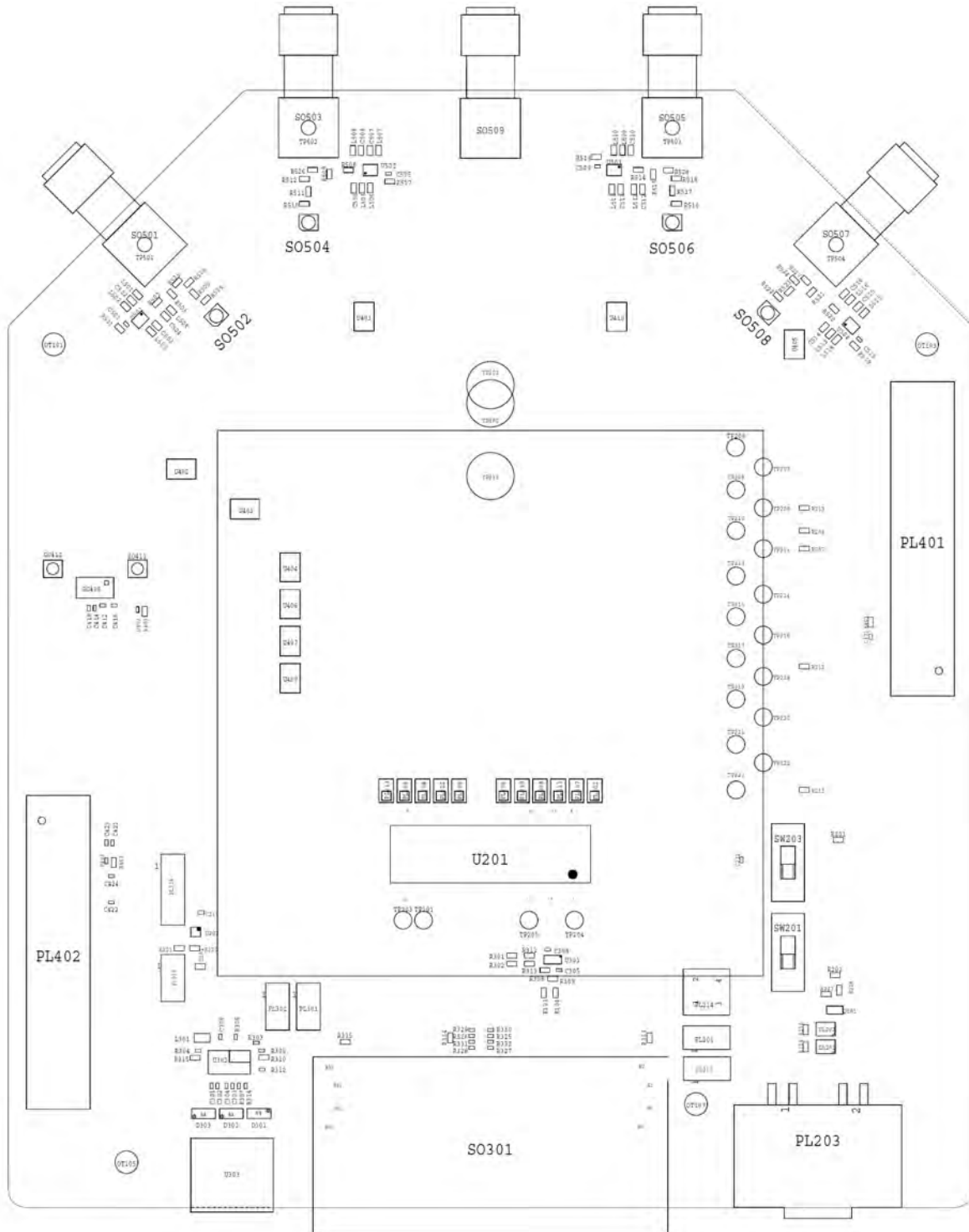
Figure 22: Component Diagram Top View
