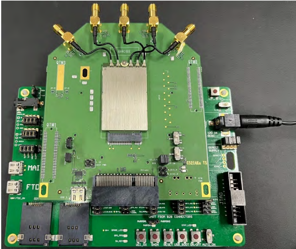
Figure 19: Connecting a wall adaptor and Telit EVB 2.0
