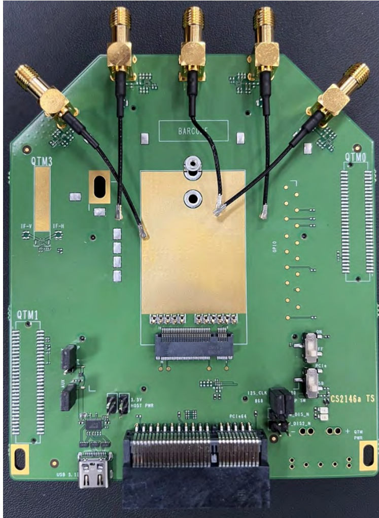
FN990 TLB Top View
