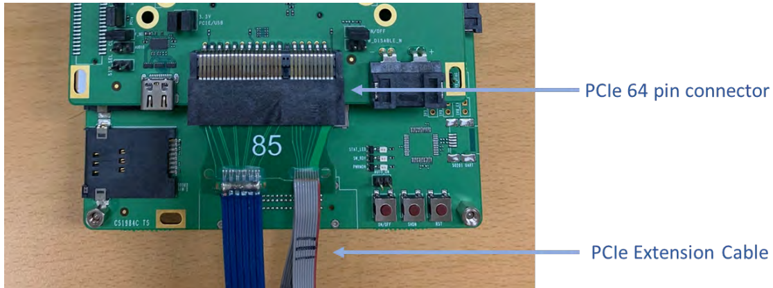
Figure 14: PCIe extension
