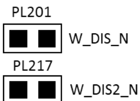
Figure 6: WLAN Disable Jumper
