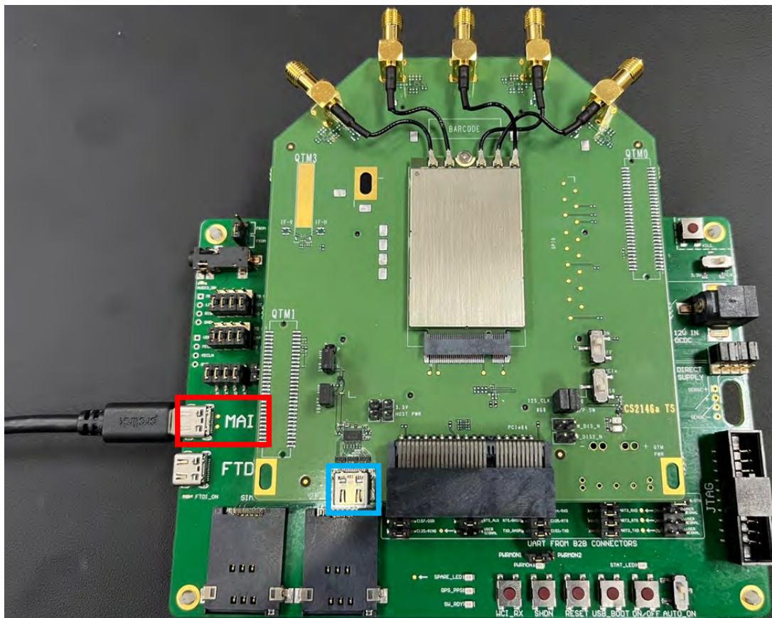
Figure 21: Connecting an USB cable and Telit EVB 2.0
