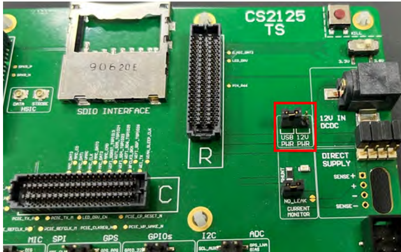
Figure 20: EVB 2.0 Jumper Setting for USB PWR mode
