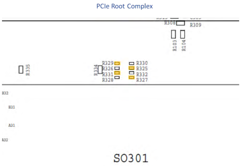
Figure 17: PCIe Root Complex
