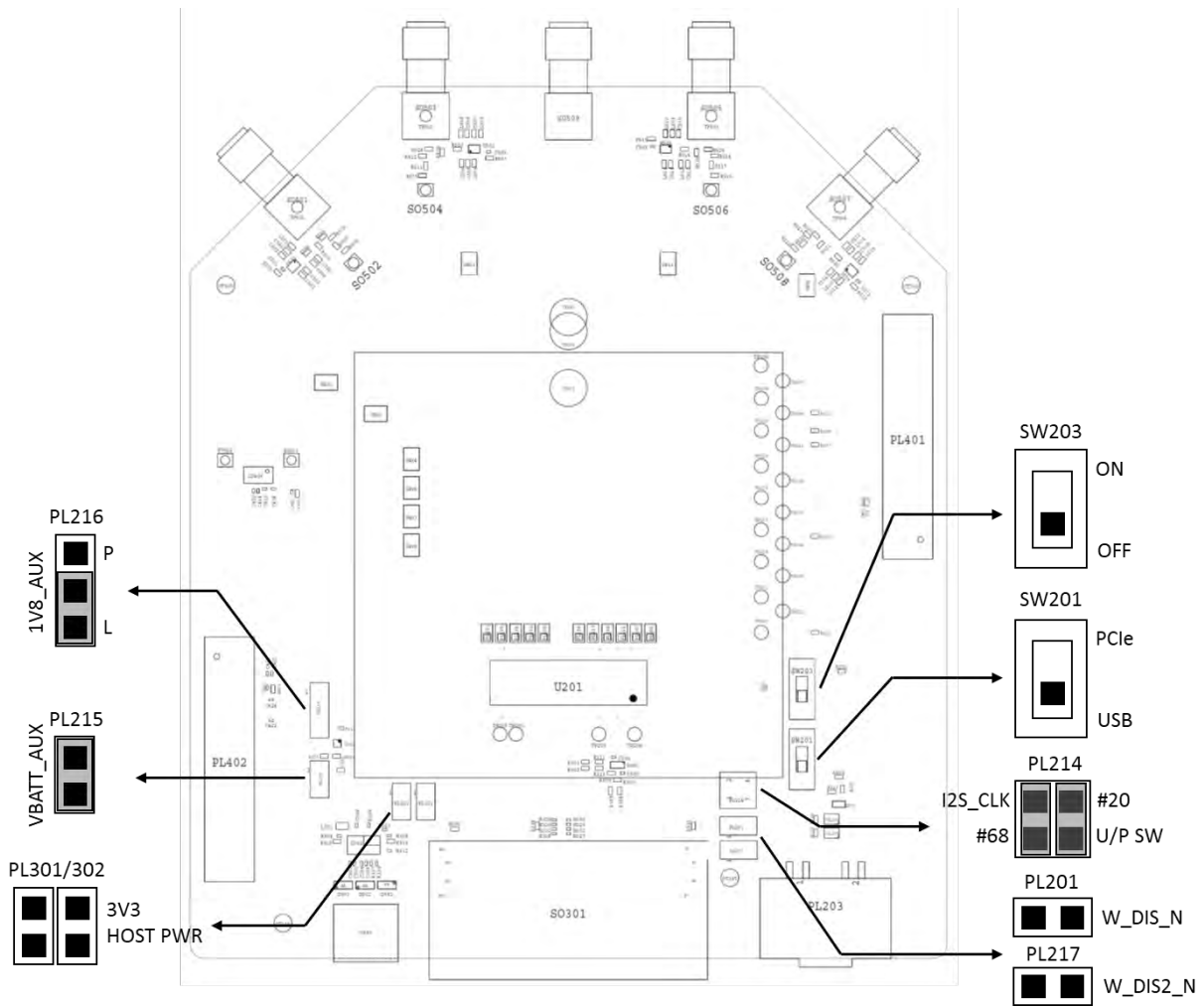
Figure 11: Default Jumper and Switch Setting of TLB with Silk
